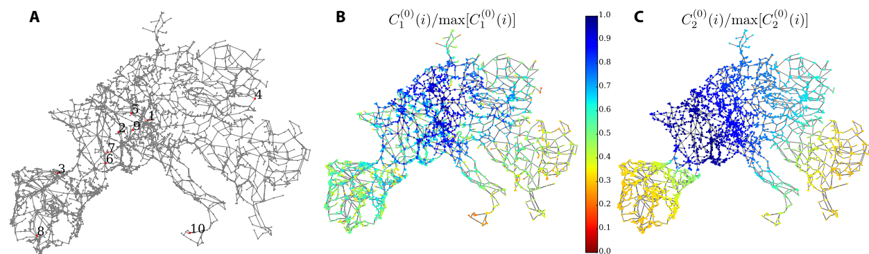
Fig. 2. Synchronous high-voltage power grid of continental Europe. (A) Topology of the European electric power grid (see Materials and Methods and the Supplementary Materials) and location of the 10 test nodes listed in Table 1. Normalized generalized resistance centralities C_1^{(0)}(i) (B) and C_2^{(0)}(i) (C) for the network Laplacian matrix of the European electric power grid.
