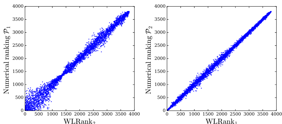
Fig. 6. Comparison between WLRank and numerical ranking for systems with inhomogeneous inertia and damping parameters. (Left) Numerically obtained ranking based on the performance measure \mathcal{P}_1 plotted against the ranking WLRank 2 based on the centrality C_2 and (right) numerically obtained ranking based on the performance measure \mathcal{P}_2 plotted against the ranking WLRank 1 based on the centrality C_1 . Each point is an average *over* more than 40 different noisy disturbances on a single node of the European electric power grid sketched in Fig. 2A, with independently fluctuating damping and inertia coefficients, d_i = d_0 + \delta d_i and m_i = m_0 + \delta m_i with \delta m_i/m_0, \delta d_i/d_0 \in [-0.4, 0.4] and \gamma = d_0/m_0 = 0.4 \text{ s}^{-1} . The noise correlation time is given by \gamma\tau_0 = 4 .
